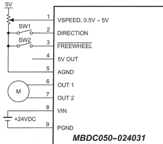
Figure 1: Hook Up for External Voltage Speed Control
